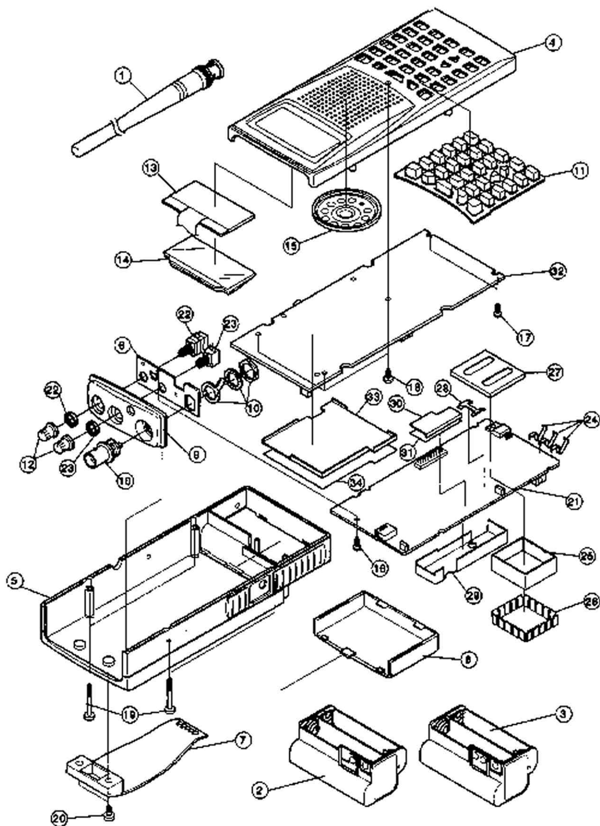
MODEL PRO-93 300-CHANNEL PORTABLE TRUNKING SCANNER EXPLODED VIEW (200-0523) FAXBACK DOC # 12771
