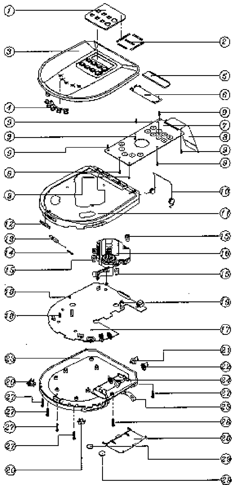
PORTABLE COMPACT DISC PLAYER EXPLODED VIEW (420-5098) FAXBACK DOC # 25410
