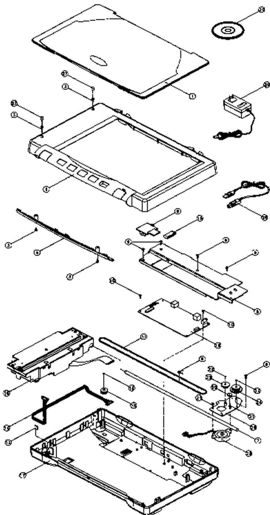
USB FLATBED SCANNER EXPLODED VIEW (250-3053) FAXBACK DOC # 12772
